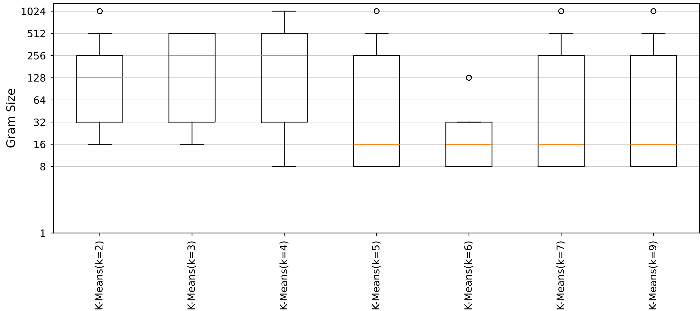
YARA Rules Gram Size Distribution (Cluster11_Size9 dataset)
